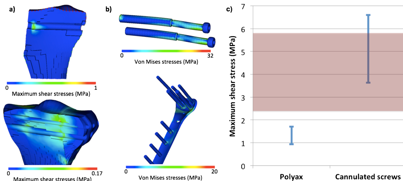
Fig. 5 Stress distributions in different parts of the deformed finite element models (deformations magnified x100). a) Model frontal cuts that shows the trabecular bone maximum shear stresses around the screws of the cannulated screw ( top ) and Polyax® ( bottom ) systems. (Colour dots at the cranial and lateral model periphery on the top
